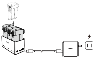
Taking LKTOP 100W Mini 5 Pro Two-Way Charging Hub +LKTOP 100W Charger as an Example
