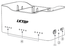
①Function Button ②Mode Indicator ③USB-C Input/Output Port ④Battery Status Indicator
